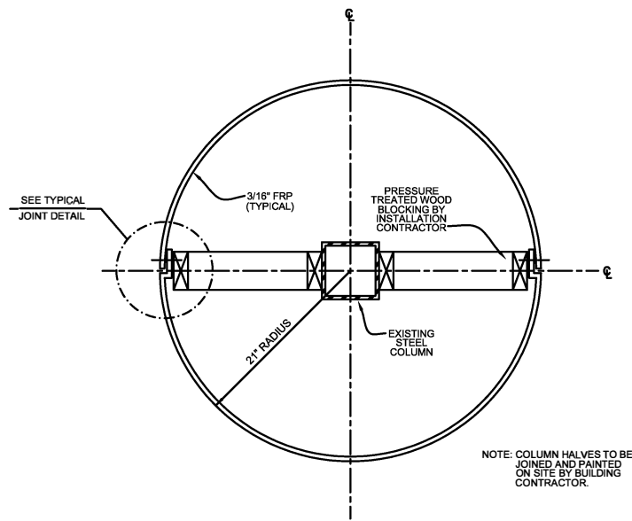
2 F2 TYPICAL SPLIT COLUMN SECTION NOT TO SCALE
