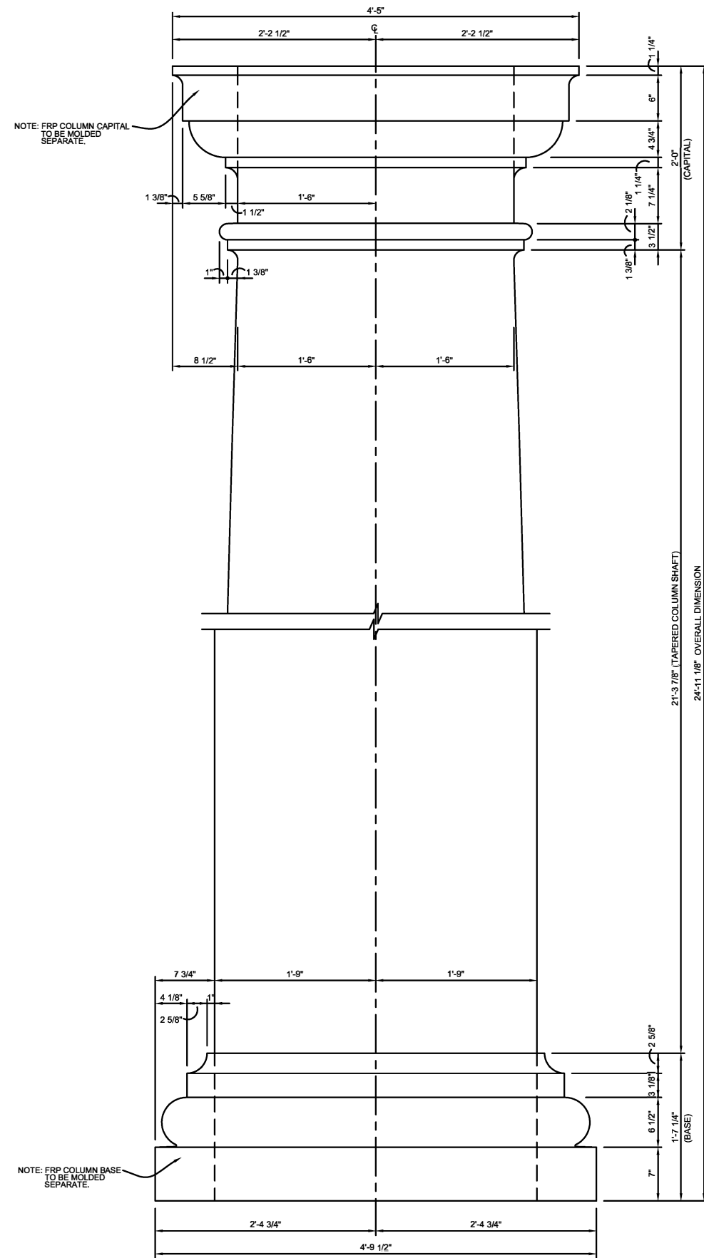
1 F2 ELEVATION - 42\"/> NOTE: ALL FRP COLUMNS TO BE SUPPLIED UNFINISHED WITH SINGLE COLOR GEL COAT. (PRIMER AND FINAL PAINT TO BE APPLIED IN FIELD BY OTHERS)
