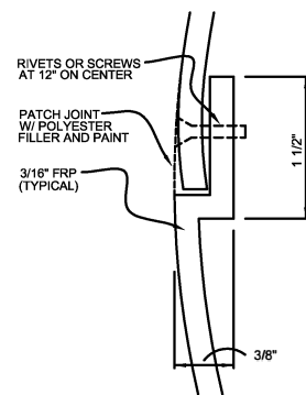
3 F2 TYPICAL VERTICAL JOINT DETAIL FULL SCALE
