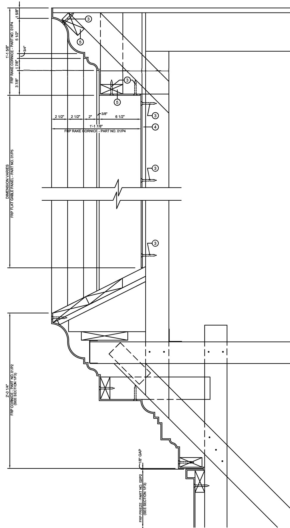
FRP RAKE CORNICE PART NO. 01/P4 FRP GABLE PANEL PART NO. 01/P5 SECTION - FRP RAKE CORNICE AND GABLE PANEL SCALE: 3"=1'-0" NOTE: ALL FRP CORNICE AND FRIEZE TO BE SUPPLIED UNFINISHED WITH SINGLE COLOR GEL COAT. (PRIMER AND FINAL PAINT TO BE APPLIED IN FIELD BY OTHERS)
