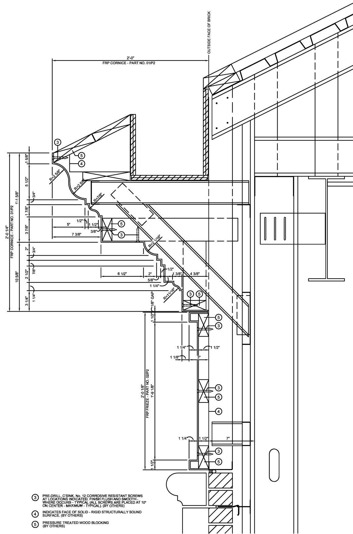
FRP CORNICE PART NO. 01/P2 FRP FRIEZE PART NO. 02/P2 SECTION - FRP CORNICE AND FRIEZE SCALE: 3"=1'-0" NOTE: ALL FRP CORNICE AND FRIEZE TO BE SUPPLIED UNFINISHED WITH SINGLE COLOR GEL COAT. (PRIMER AND FINAL PAINT TO BE APPLIED IN FIELD BY OTHERS)
