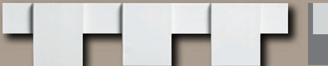
MD 1092 • 1 1/2" Projection • 4 1/2" Height • 11'8" Length • 3 1/2" Dentil • 6 1/8" Repeat
