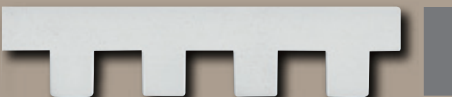
MD 1070 • 1" Projection • 3" Height • 12'0" Length • 1 1/2" Dentil • 3" Repeat
