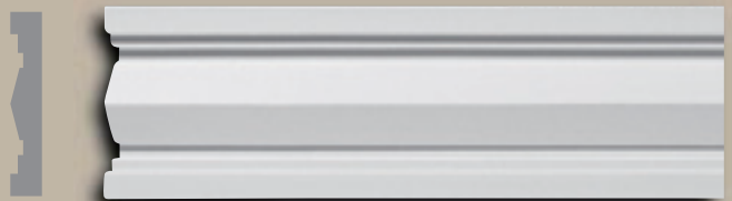
MD 1177 • 1 1/16" Projection • 6 3/16" Height • 12'0" Length
