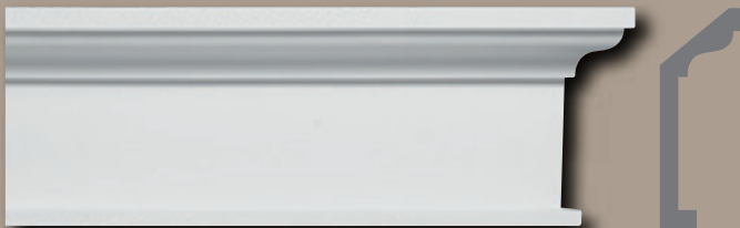
MD 1066 • 4 1/2" Projection • 12" Height • 12'0" Length
