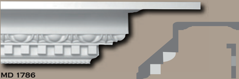
MD 1786 • 20" Projection • 12" Height • 12'0" Length • 4 15/16" Repeat
