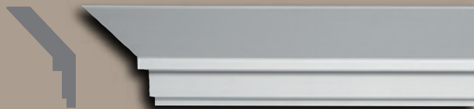
MD 1664 • 3 3/4" Projection • 4 9/16" Height • 12'0" Length
