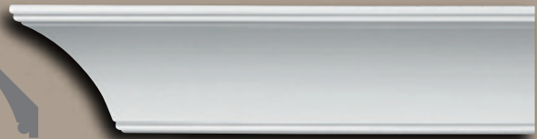
MD 1139 • 5 1/4" Projection • 5 1/4" Height • 12'0" Length
