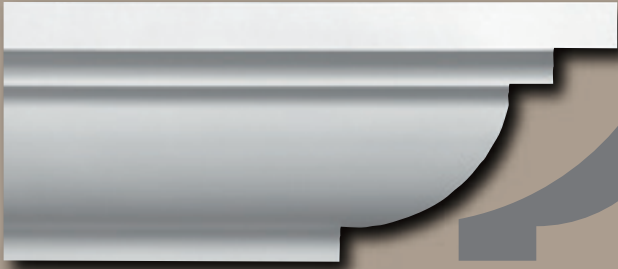
MD 1551 • 18" Projection • 15" Height • 12'0" Length
