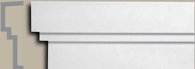
MD 1791 • 5 1/2" Projection • 17" Height • 12'0" Length
