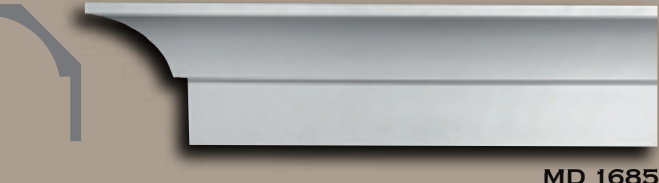
MD 1685 • 7 3/4" Projection • 12 3/4" Height • 12'0" Length
