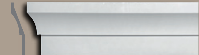
MD 1702 • 5" Projection • 19" Height • 12'0" Length
