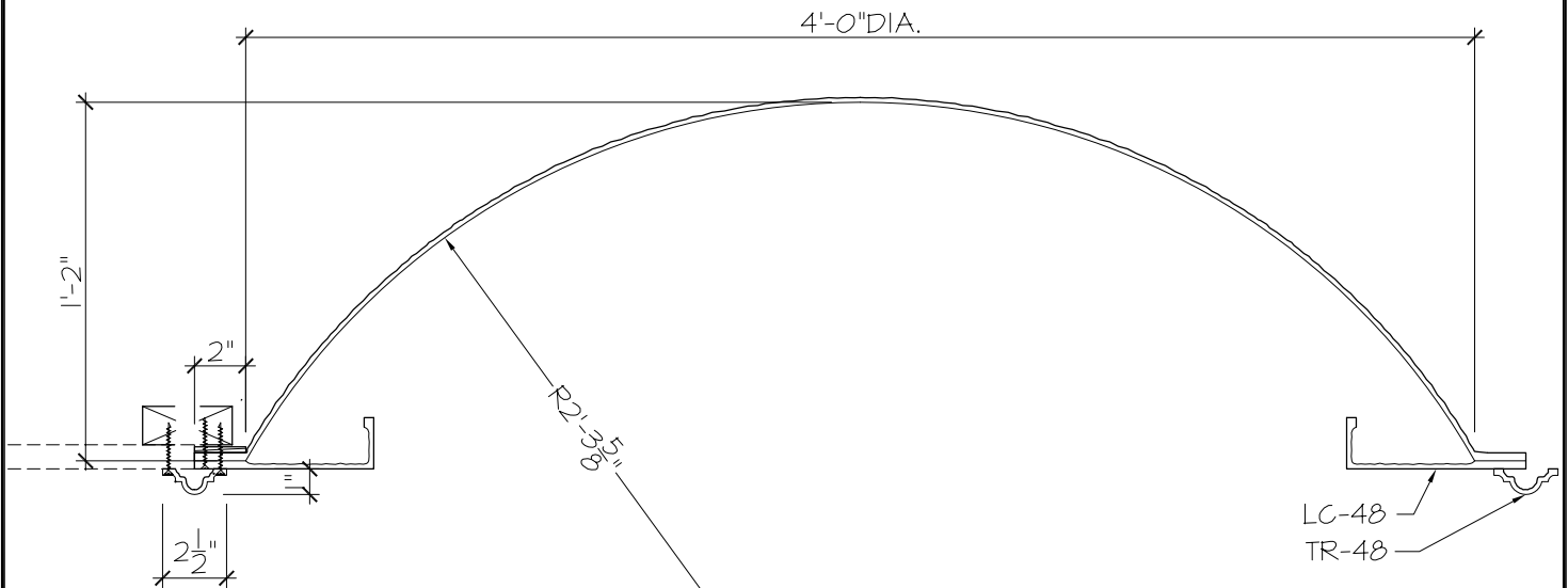
1B DETAIL SECTION SCALE : 1-1/2" = 1'-0"
