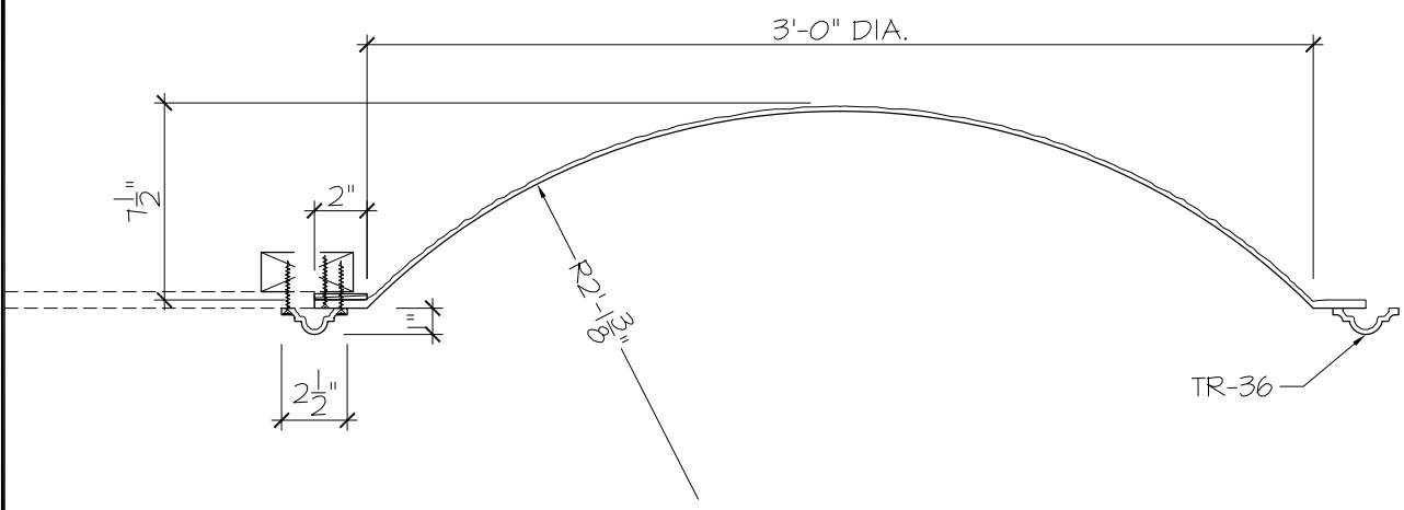
1B DETAIL SECTION SCALE : 1-1/2" = 1'-0"
