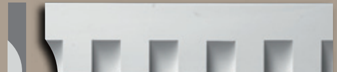
MD 1019 • 1 1/2" Projection • 5 7/8" Height • 12'0" Length • 4 3/4" Repeat • 2 3/8" x 2 3/4" Dentil
