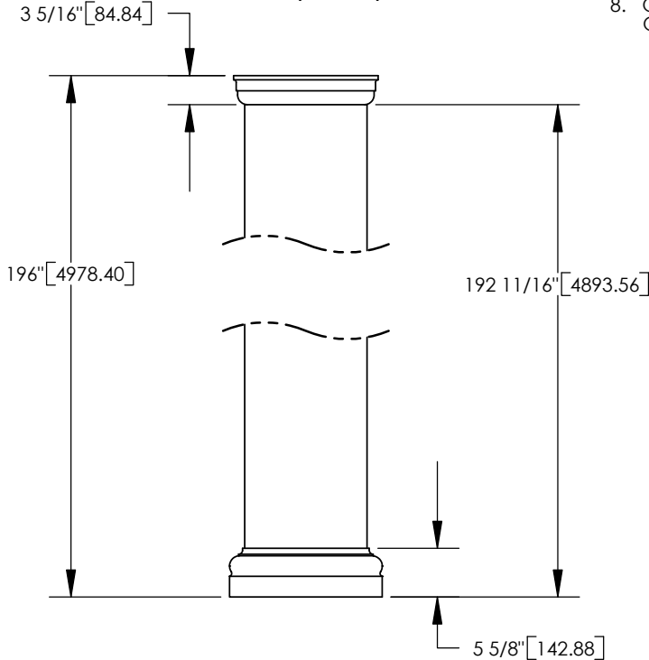
SQUARE TUSCAN 1 3/4" 1 3/4" 14" CAP
