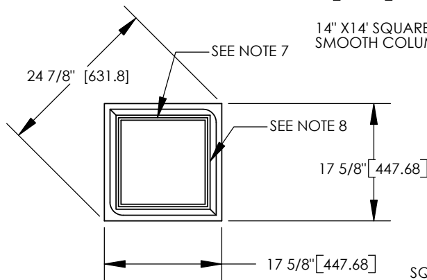
SQUARE TUSCAN 14" BASE
