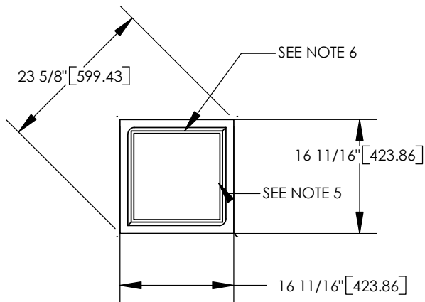
SQUARE TUSCAN 14" CAP
