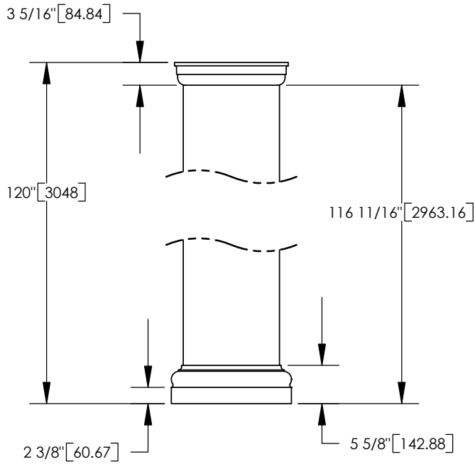
SQUARE TUSCAN 14" CAP
