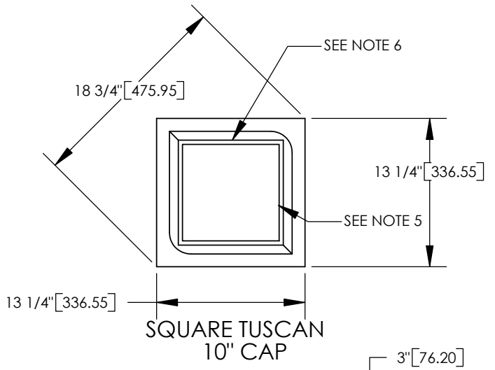
SQUARE TUSCAN CAP
