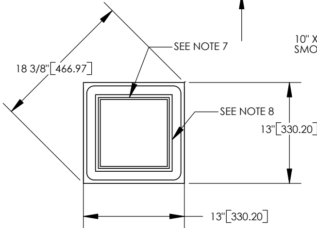
SQUARE TUSCAN 10" BASE
