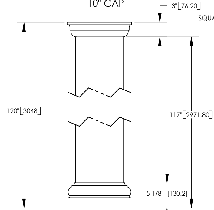
SQUARE TUSCAN 10" CAP
