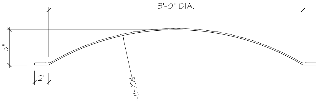
1B DETAIL SECTION SCALE : 1-1/2" = 1'-0"
